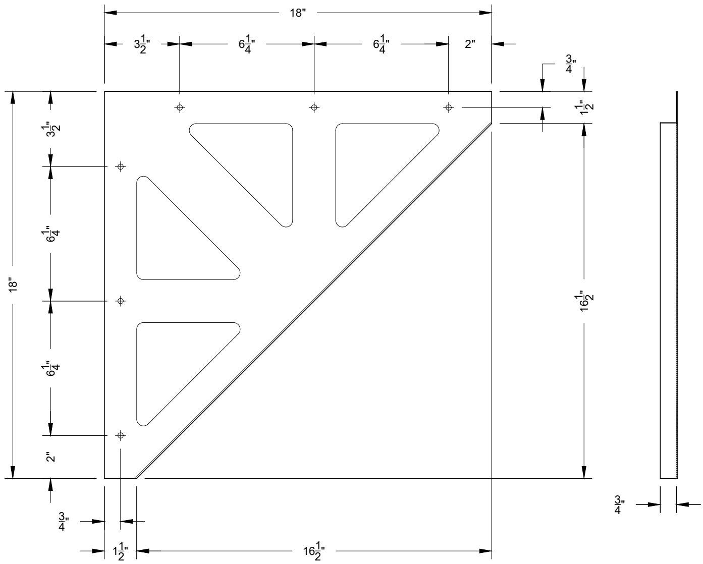
PLAN VIEW
