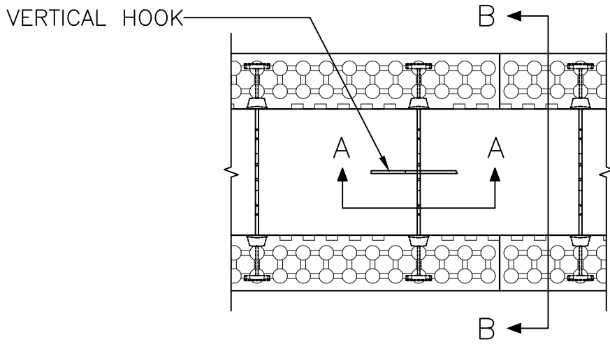
VERTICAL HOOK CONNECTING COURSES – PLAN VIEW
