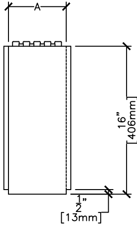
SIDE ELEVATION
