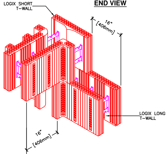
LONG T-WALL END VIEW
