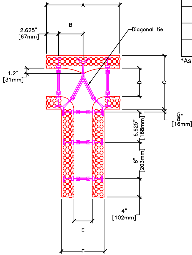
SHORT T-WALL PLAN VIEW
