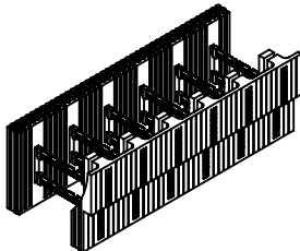
Standard—Transition Block
