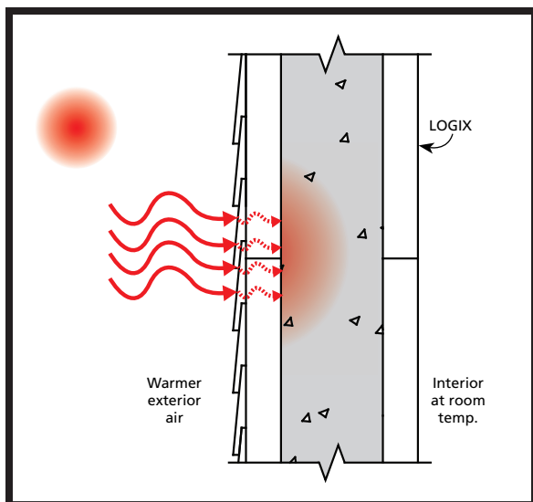
During warm summer days, heat is absorbed into the concrete core wall of LOGIX, but must first travel through a thick layer of insulation impeding the heat absorption. (See Scenario 1)
