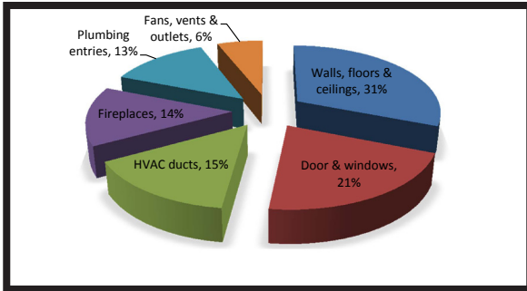
Energy loss contribution of typical residential home. Source: U.S. Department of Energy
