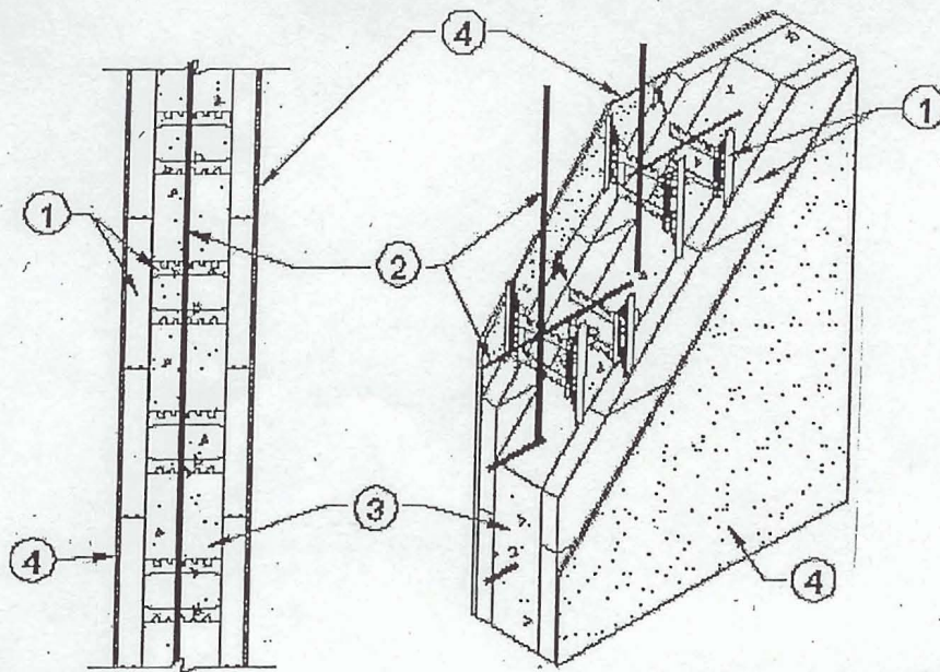
Figure 1. Logix Insulated Concrete Form wall system
