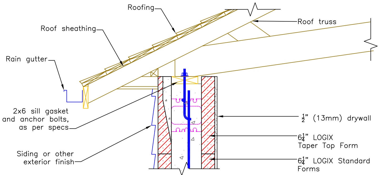
Vaulted Ceiling - Scissor Truss
