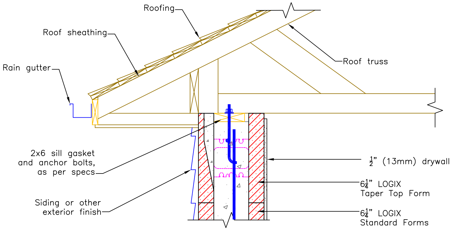
Vaulted Ceiling - A - Frame
