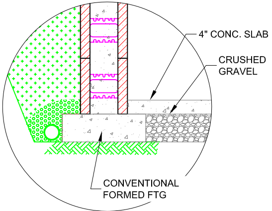
FOOTING OPTIONS
