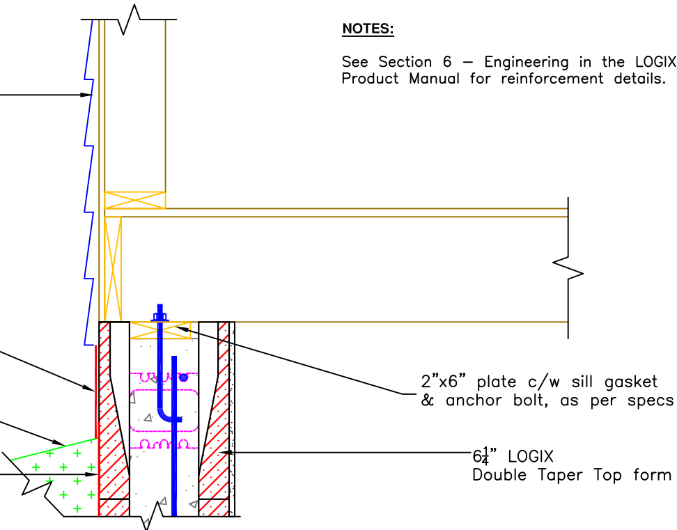
2x6 TOP PLATE RECESSED
