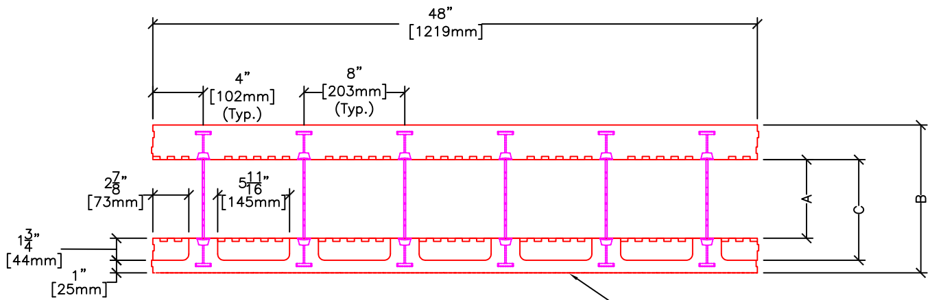
PLAN VIEW
