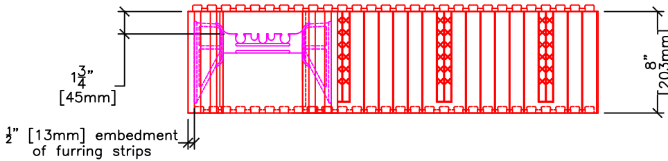
SIDE ELEVATION
