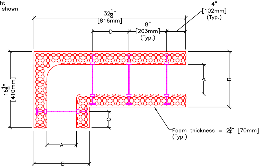
PLAN VIEW
