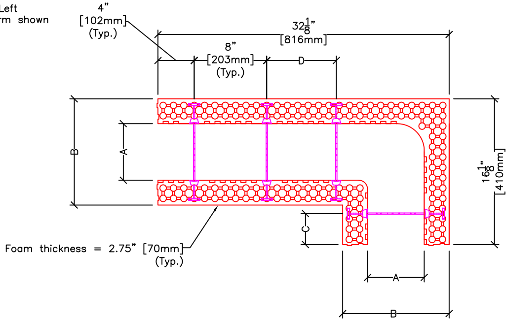
PLAN VIEW
