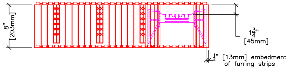
SIDE ELEVATION
