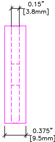
END VIEW
