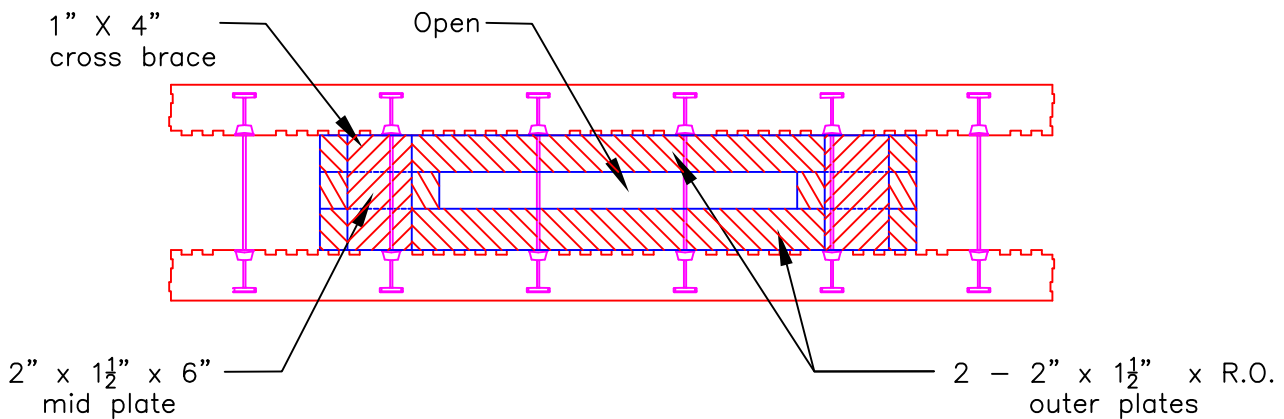
PLAN WINDOW SILL
