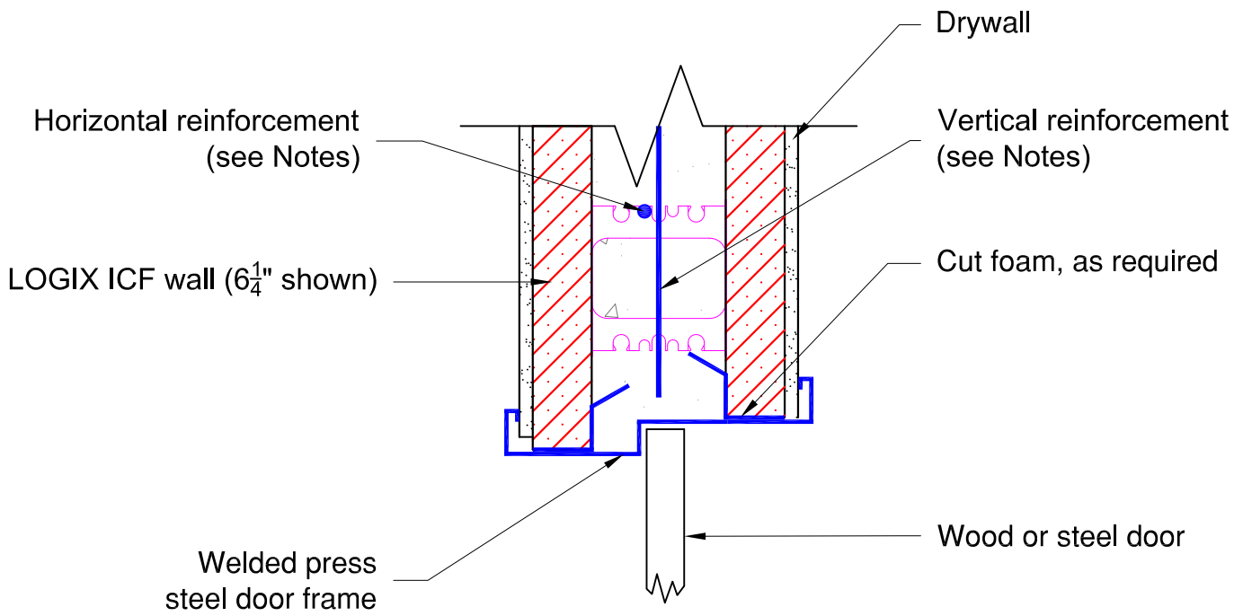
INTERIOR DOOR FRAME - HEAD CENTER MOUNTED DOOR
