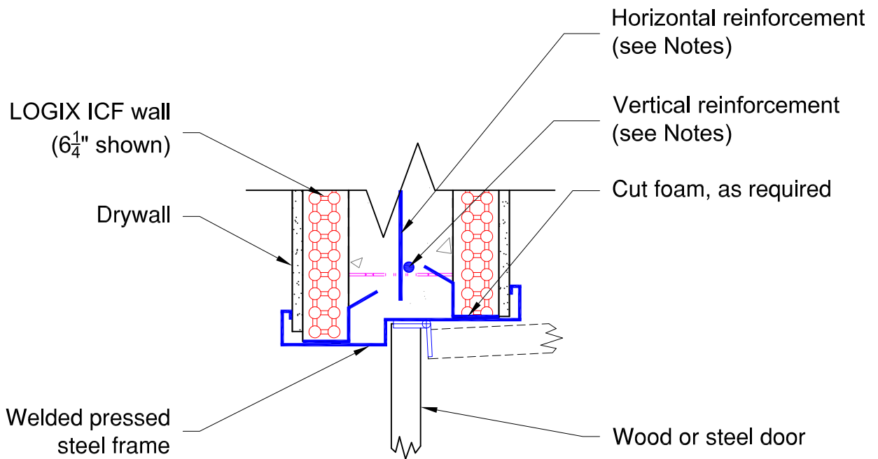
INTERIOR DOOR FRAME - JAMB CENTER MOUNTED DOOR
