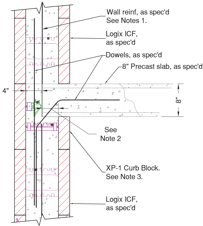
BEARING END
