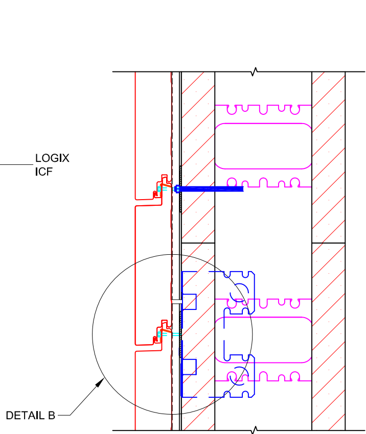
WALL SECTION AT SUBGIRTS ENDS
