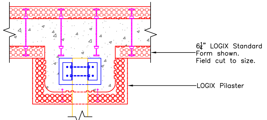
PLAN VIEW - SECTION THROUGH PILASTER (Reinforcement not shown for clarity)
