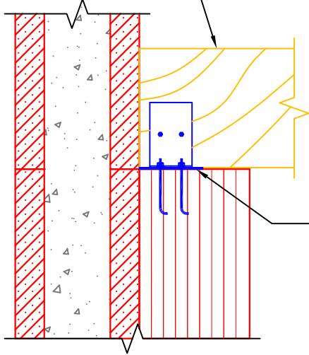
SIDE ELEVATION (Reinforcement not shown for clarity)
