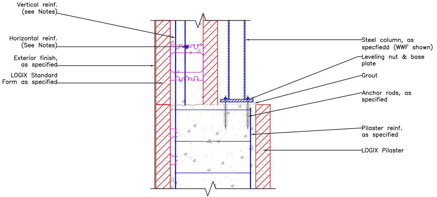
Logix Pilaster Supporting Steel Column
