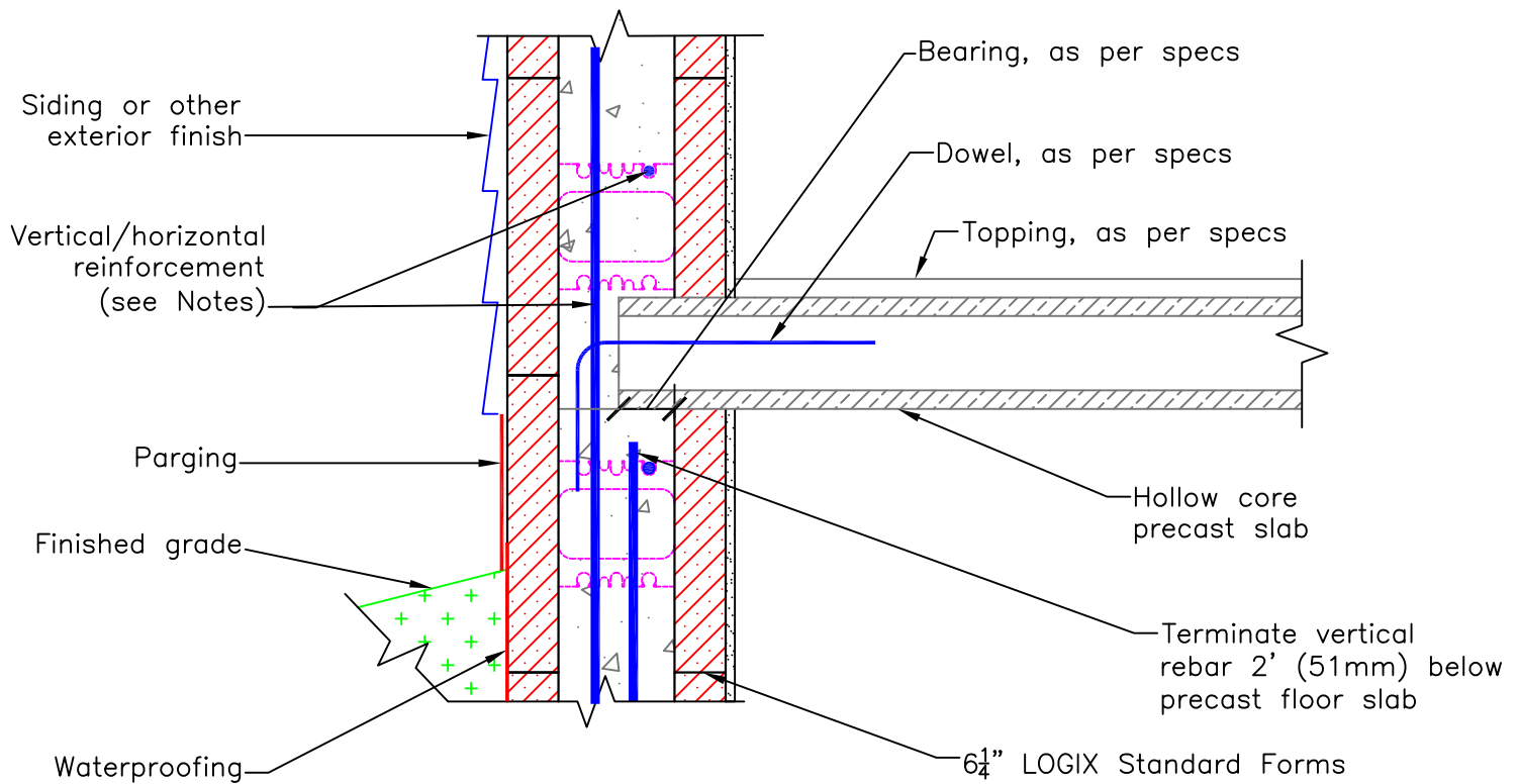
HOLLOW CORE PRECAST CONCRET SLAB (BEARING END)
