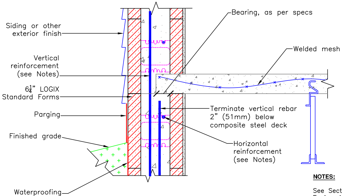
HAMBRO FLOOR SYSTEM (NON-BEARING END)
