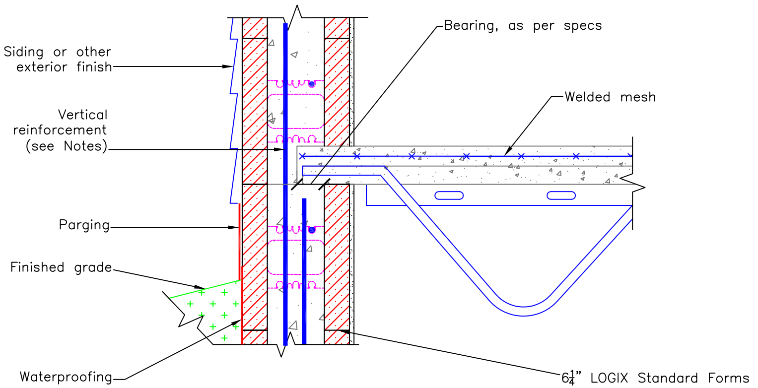
HAMBRO FLOOR SYSTEM (BEARING END)
