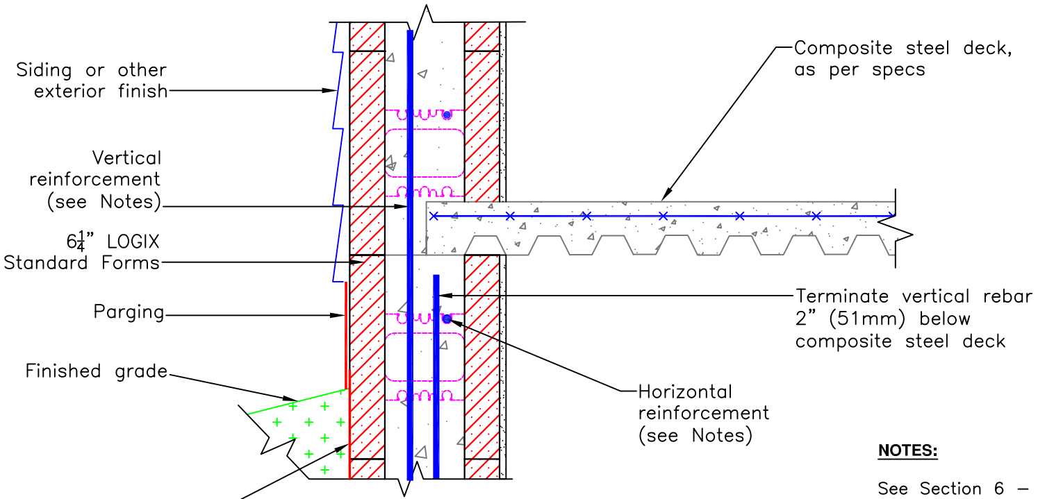
STEEL COMPOSITE DECK (NON-BEARING END)
