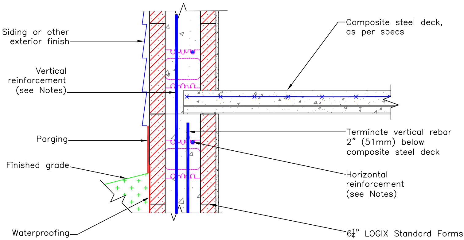
STEEL COMPOSITE DECK (BEARING END)
