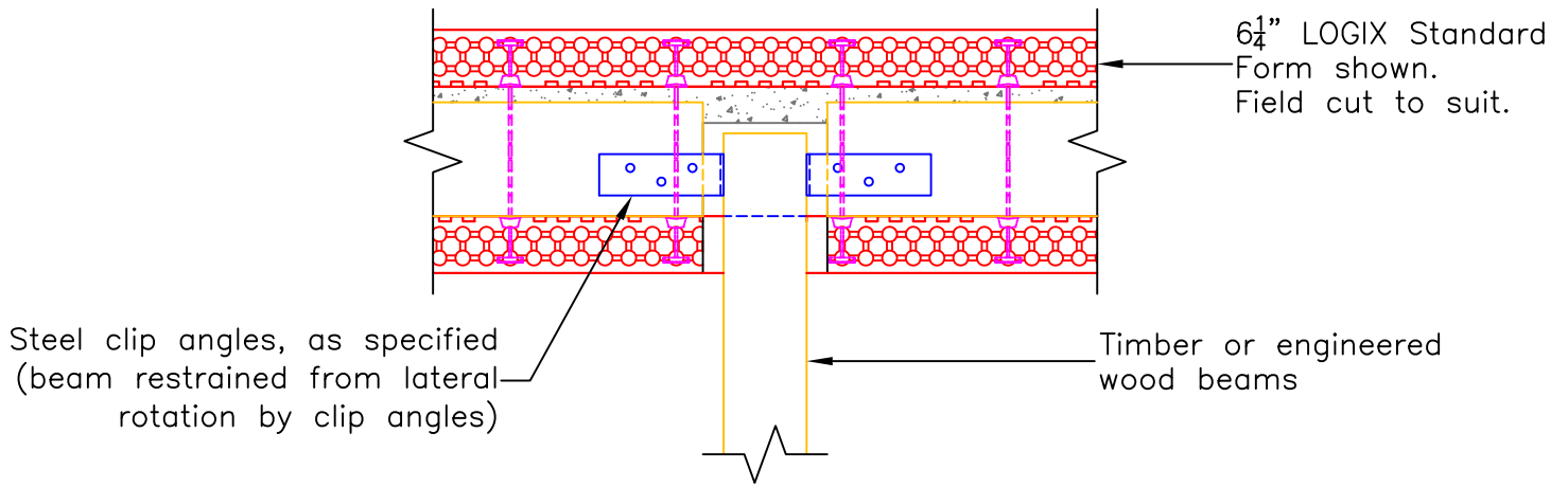
PLAN VIEW - Section at beam (Reinforcement not shown for clarity)
