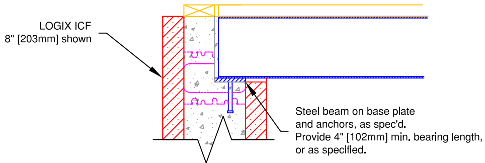
Section through Wall at Beam Pocket
