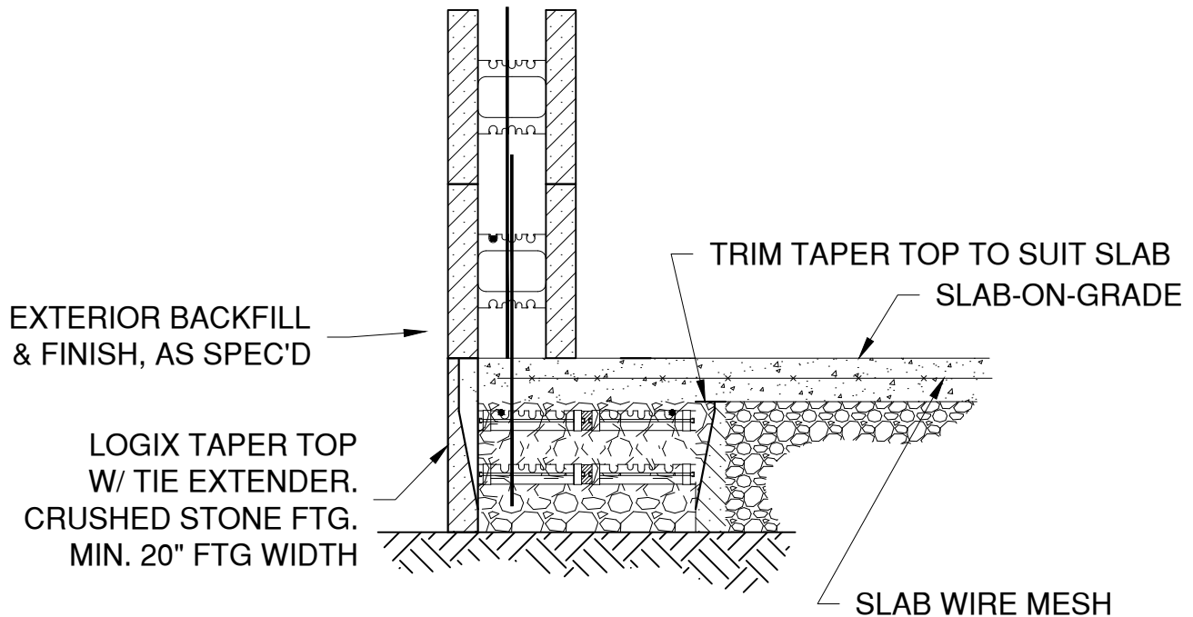
ALASKAN SLAB DETAIL WITH CONTINUOUS ICF
