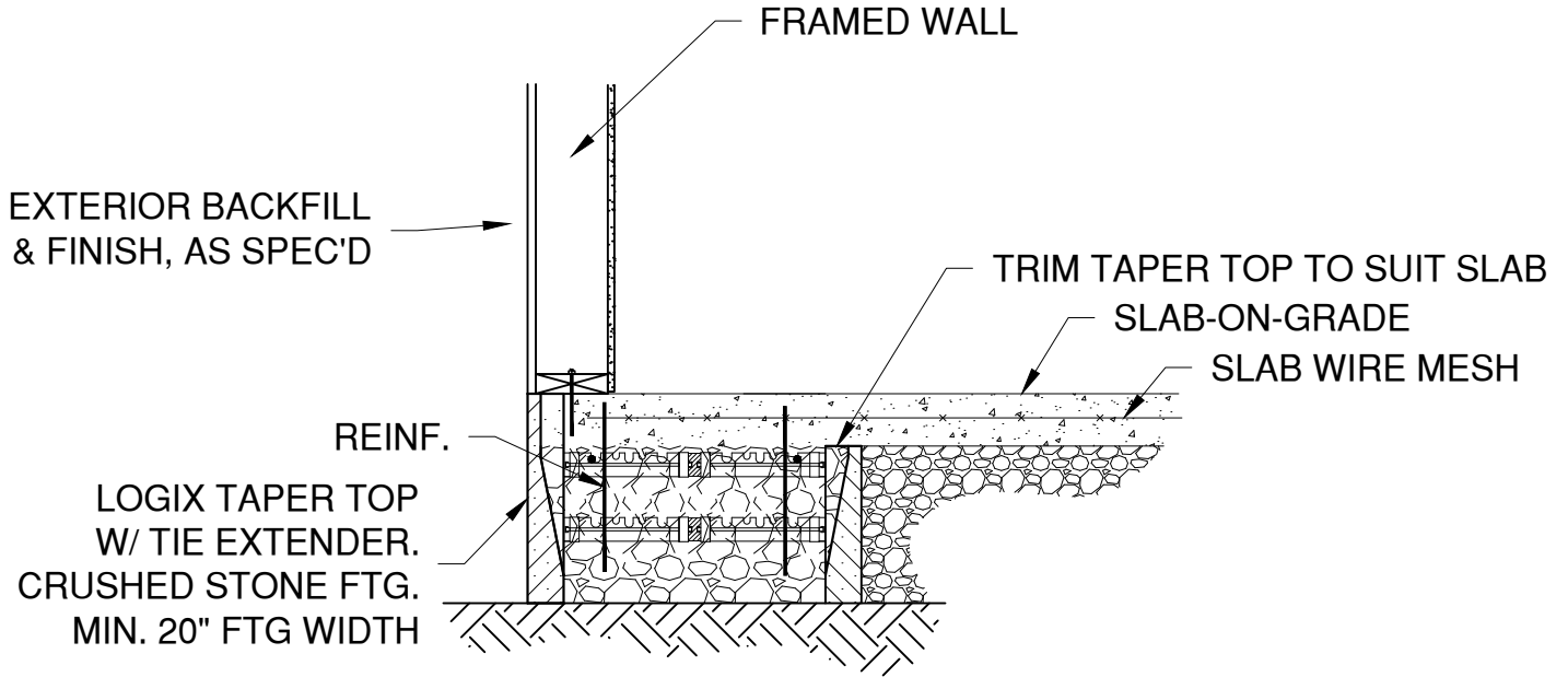
ALASKAN SLAB DETAIL WITH FRAMED WALL
