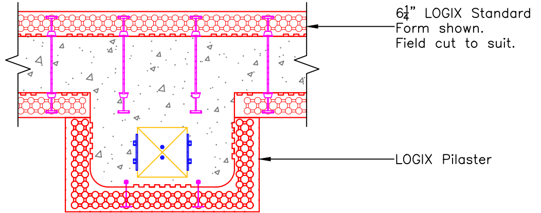
PLAN VIEW (Reinforcement not shown for clarity)
