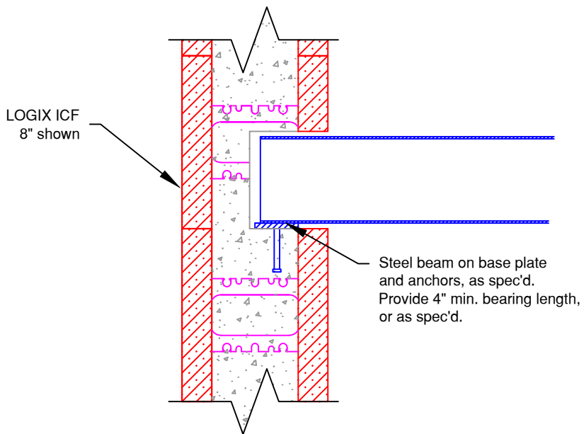
Section through Wall at Beam Pocket
