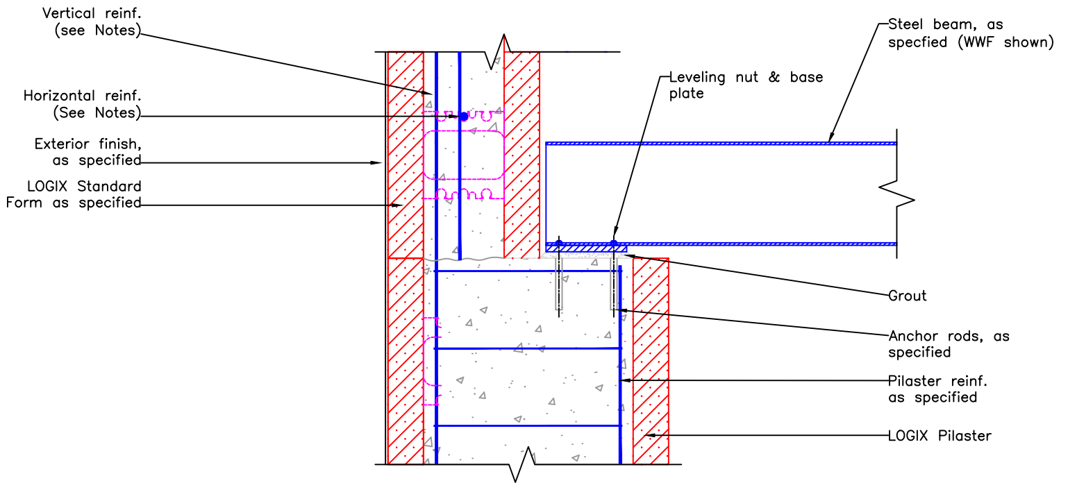
Logix Pilaster Supporting Steel Beam
