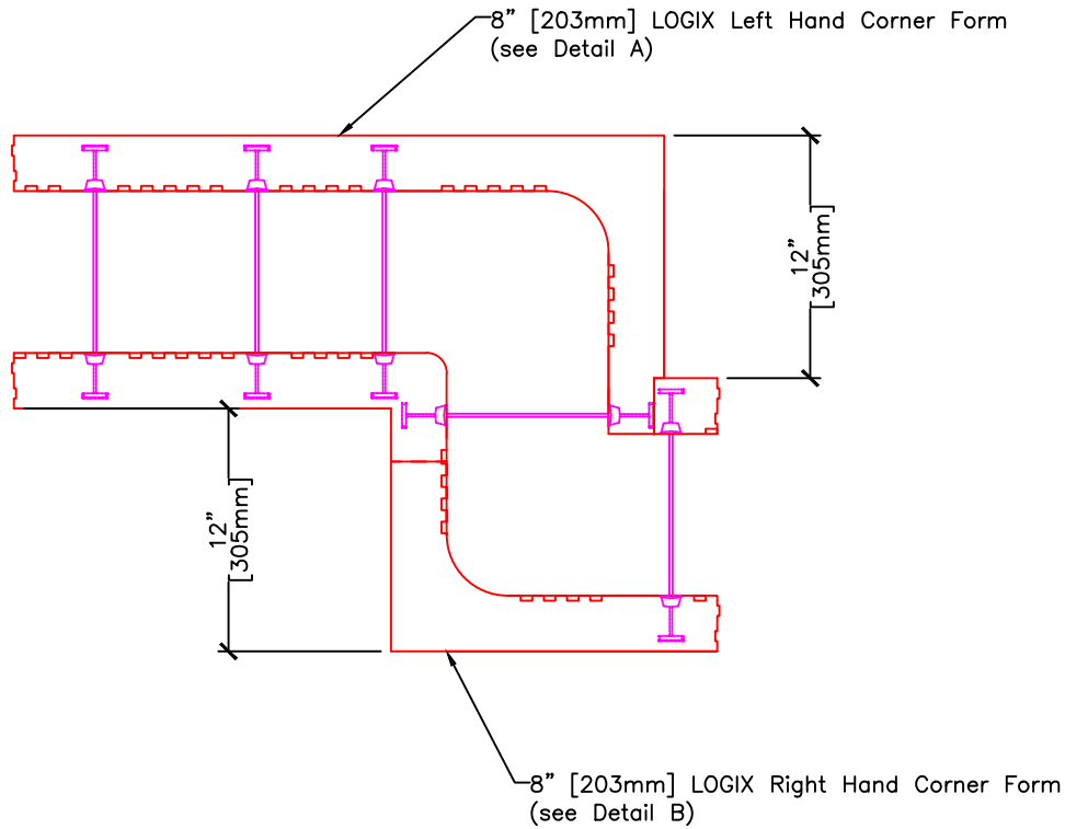
PLAN VIEW
