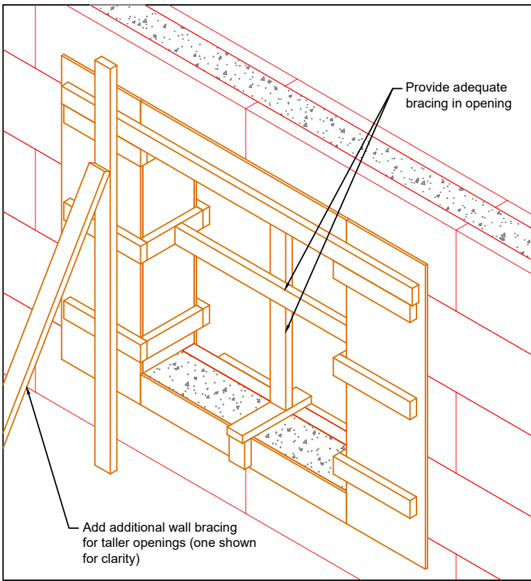
FORM SUPPORT - EXTERIOR SIDE
