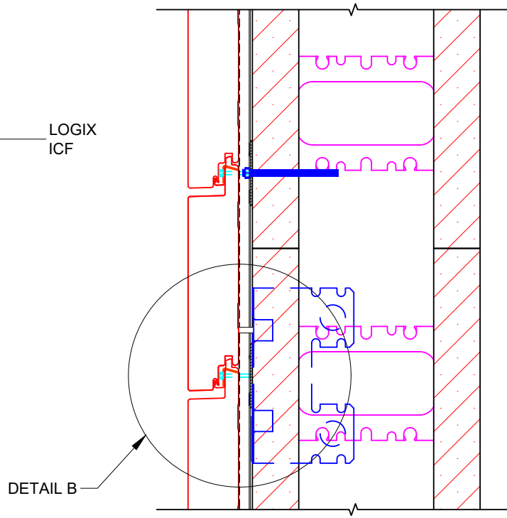
WALL SECTION AT SUBGIRTS ENDS
