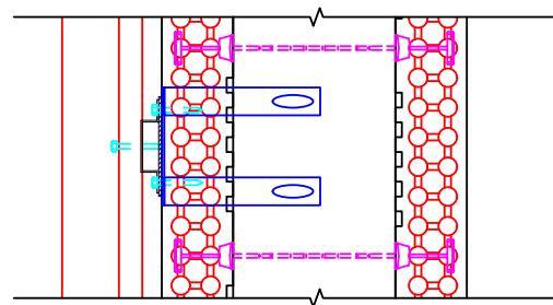
PLAN VIEW SHOWING SIMPSON CONNECTOR AT SUBGIRT ENDS
