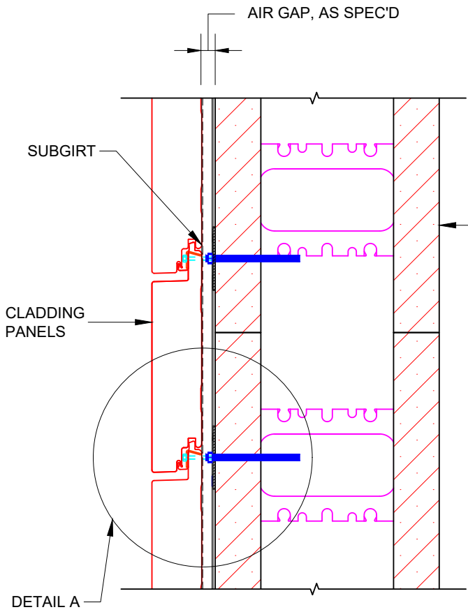
WALL SECTION ALONG SUBGIRTS
