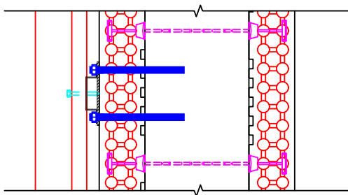
PLAN VIEW SHOWING EXPANSION ANCHORS ALONG SUBGIRT
