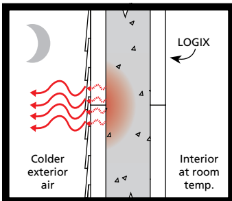
At night temperatures fall below the interior temperature, which causes the heat absorbed during the day to flow to the colder exterior side of the wall. (See Scenario 1)
