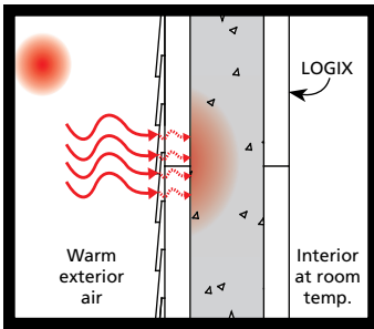
During warm summer days, heat is absorbed into the concrete core wall of LOGIX, but must first travel through a thick layer of insulation impeding the heat absorption. (See Scenario 1)
